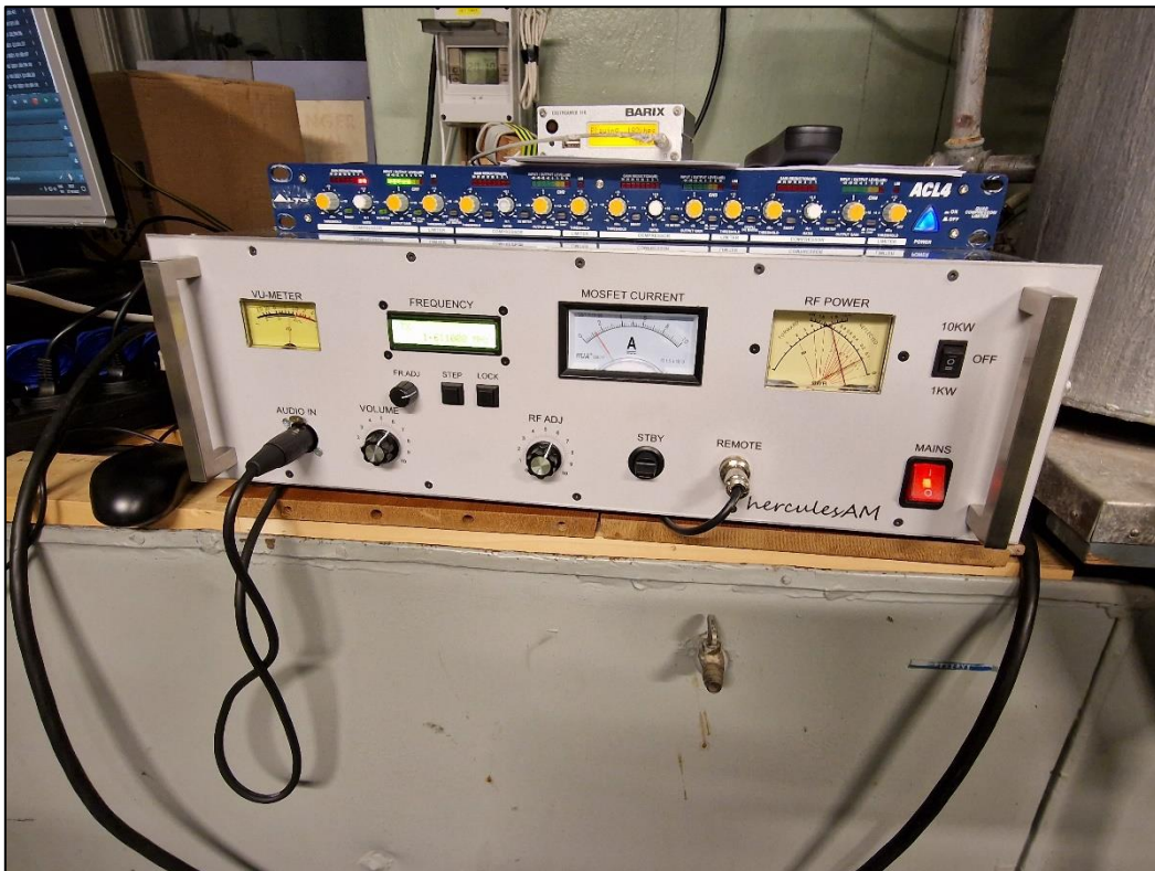
2 kW Hercules transmitter of which 400 watts is regularly used. (Northern Star Media Services AS)
