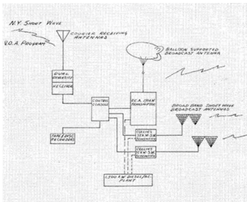
Balloon electronics. Unknown artist. Perhaps issued by the VOA.
