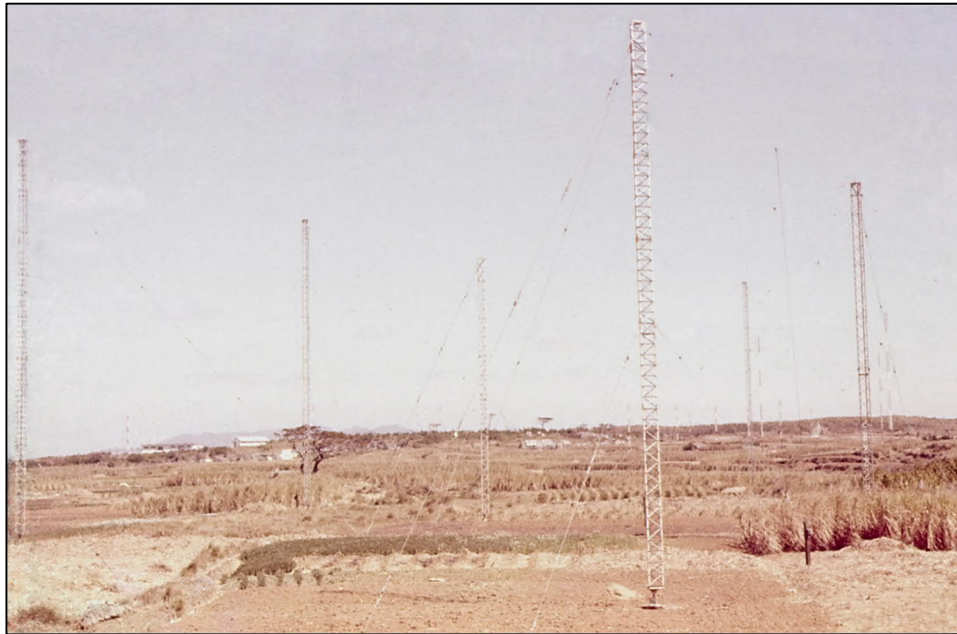
Part of the antenna field with the VoA relay station in the background 1963
