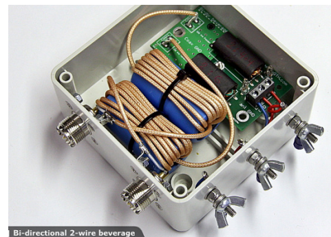
Bi-directional 2-wire beverage
